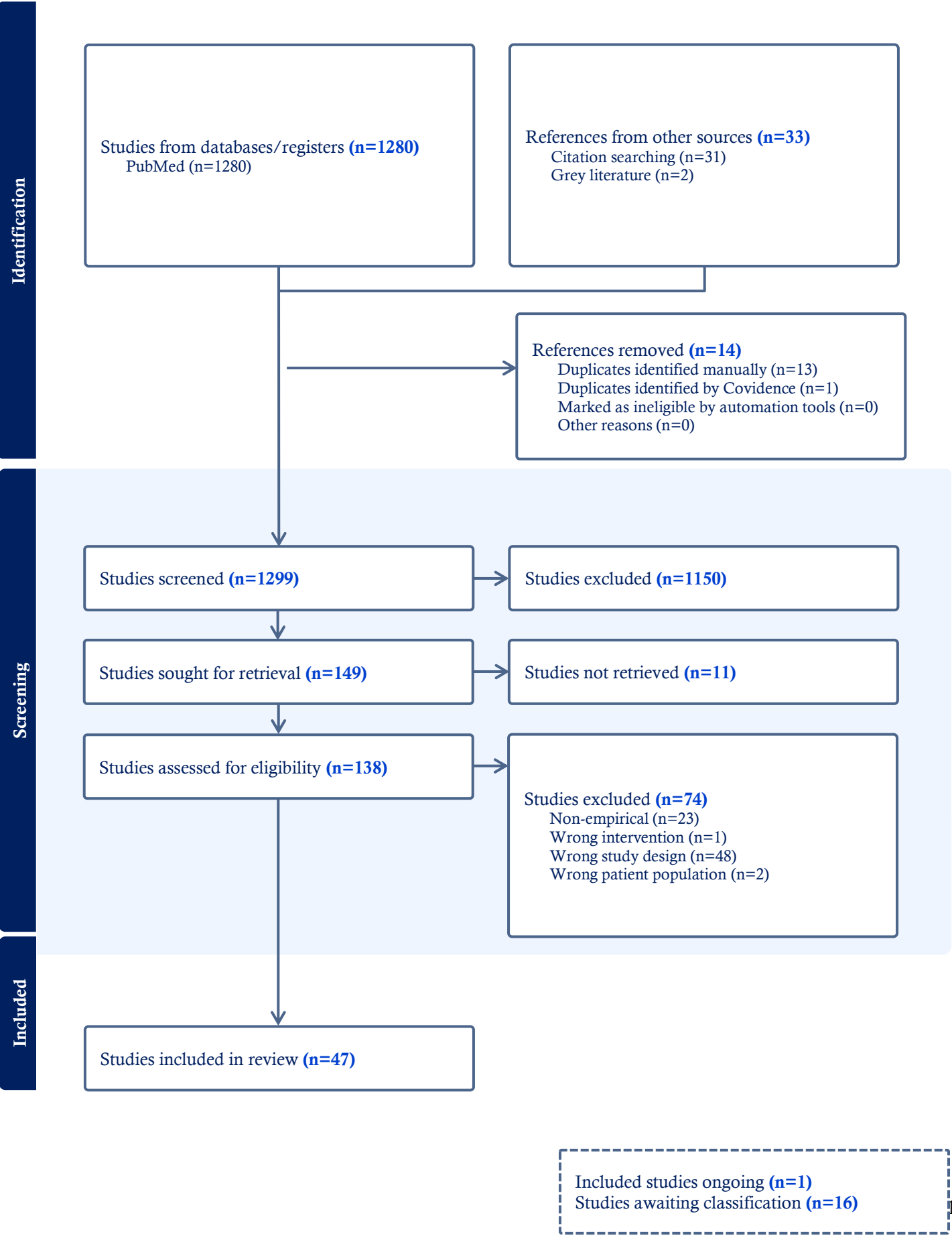
Figure 1. PRISMA chart
